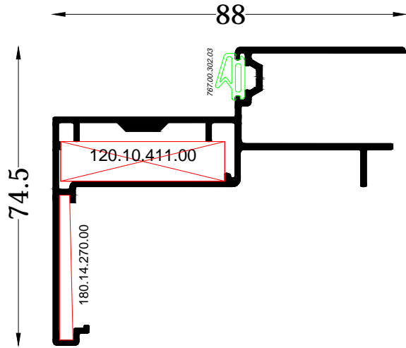
M0194 Linear frame for wooden panel sash 42mm
