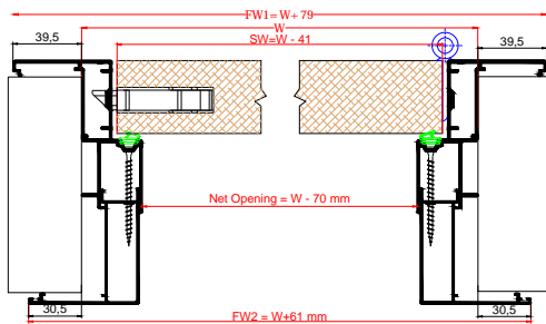
Linear Twin Door M0192 or M194 + M0070
