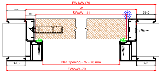
Linear Twin Door M0192 or M0194 + M0193
