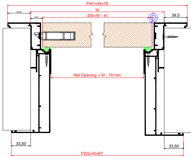
Linear Twin Door M0192 or M0194 + M0186
