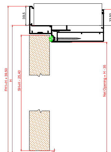
Linear Twin Door M0192 or M0194 + M0185
