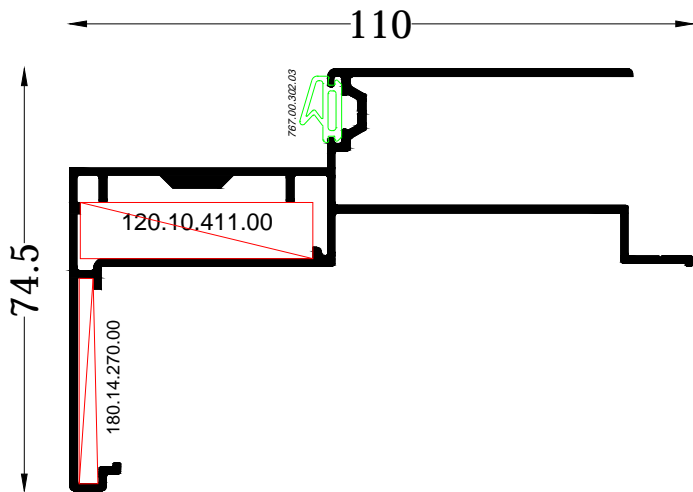
M0192 Linear frame for wooden panel sash 42mm
