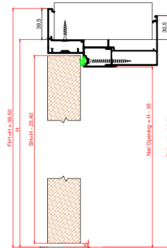
Linear Twin Door M0192 or M194 + M0070
