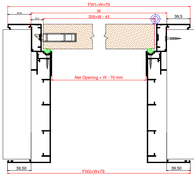
Linear Twin Door M0192 or M0194 + M0187
