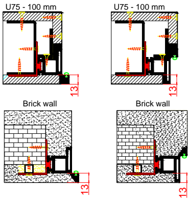
OPENING INSIDE OPENING OUTSIDE
